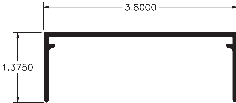
Series 4, 4" Frameless Body Part #1355
